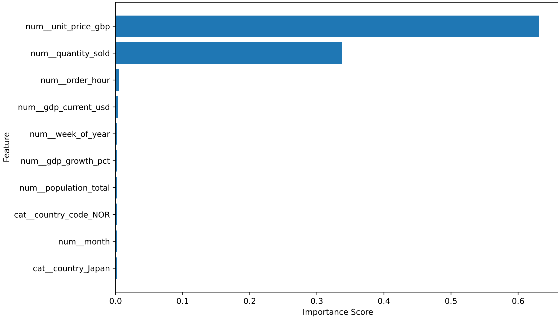
RQ4 - Top 10 Important Features
